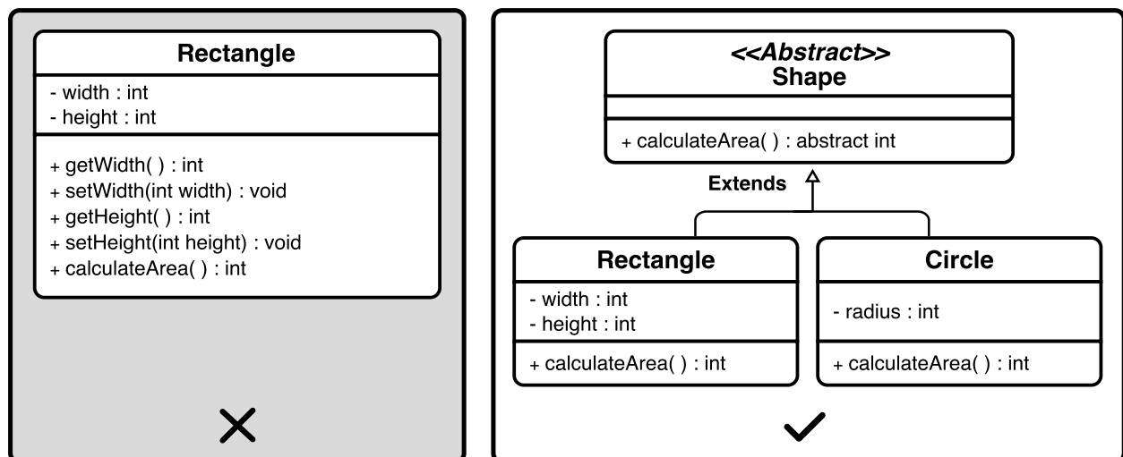
Open/Closed Principle (OCP)
