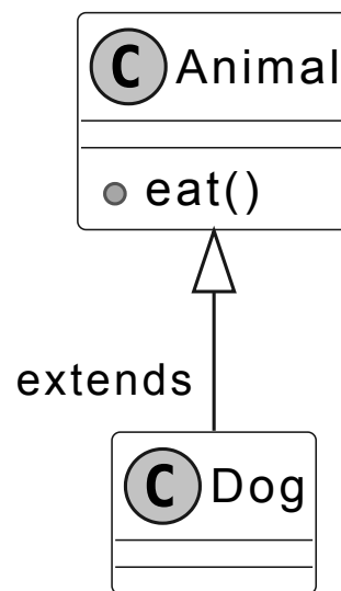
Single inheritance
