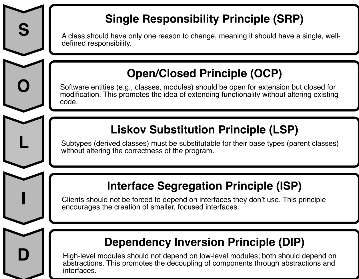
SOLID Principles
