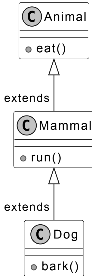
Multilevel inheritance
