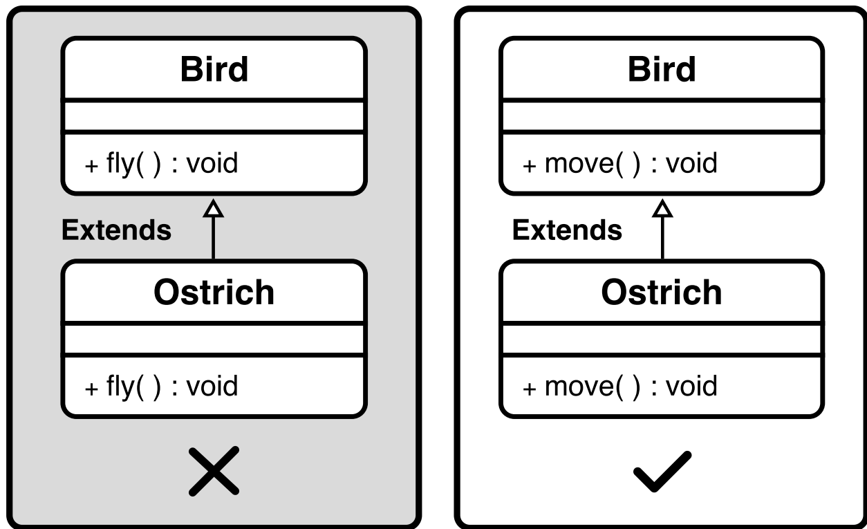
Liskov Substitution Principle (LSP)
