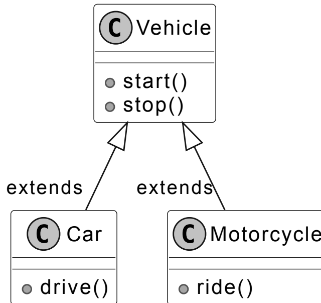
Hierarchical inheritance
